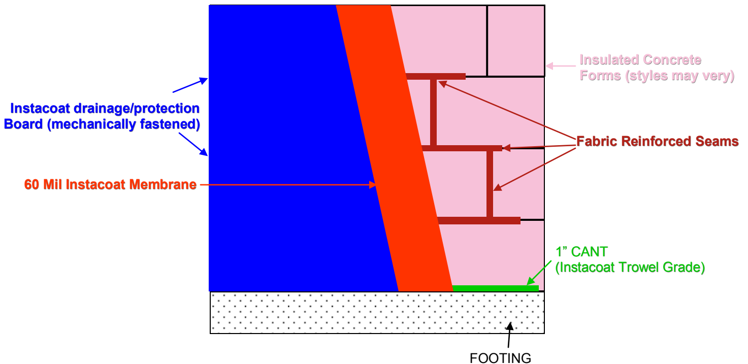
SIDE VIEW
