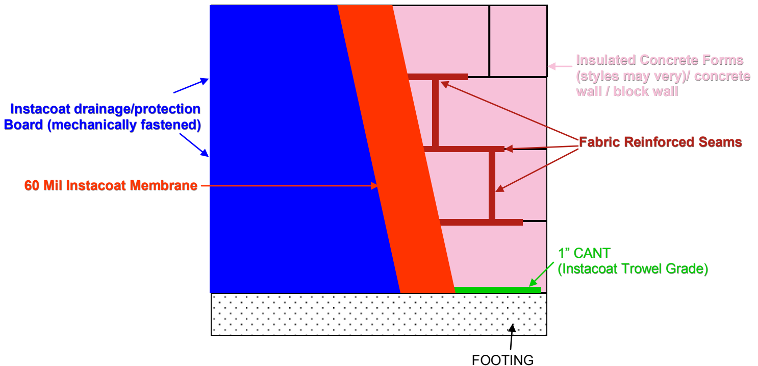
SIDE VIEW
