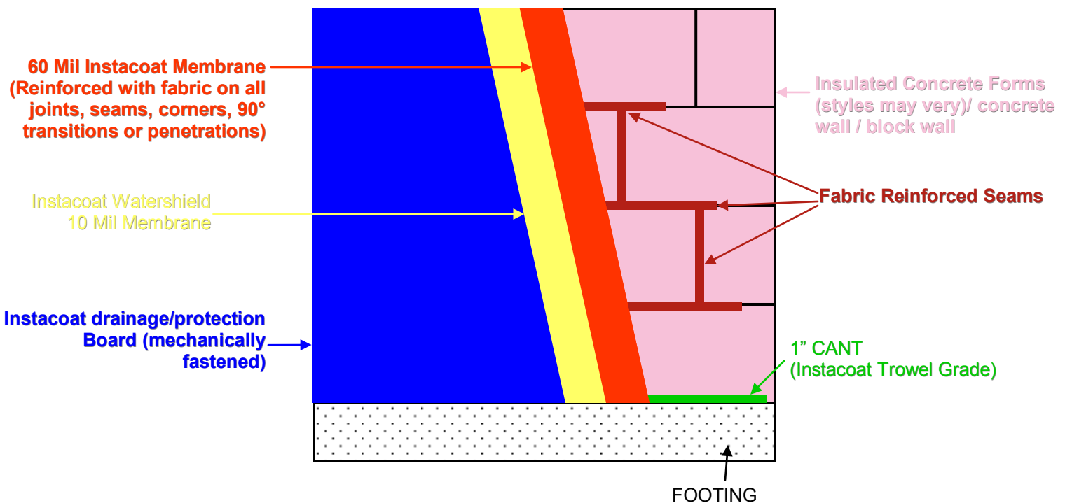
SIDE VIEW
